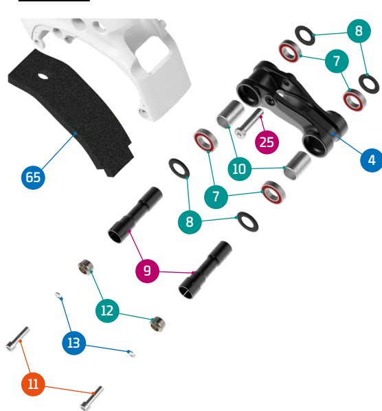
DETAIL 02
