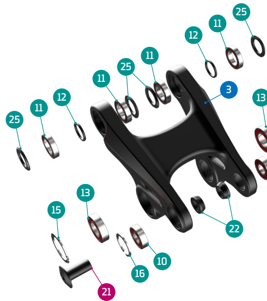
DETAIL 01
