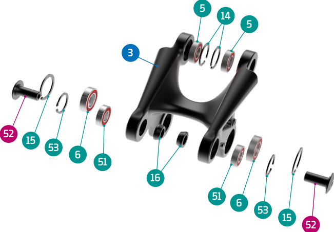
DETAIL 01
