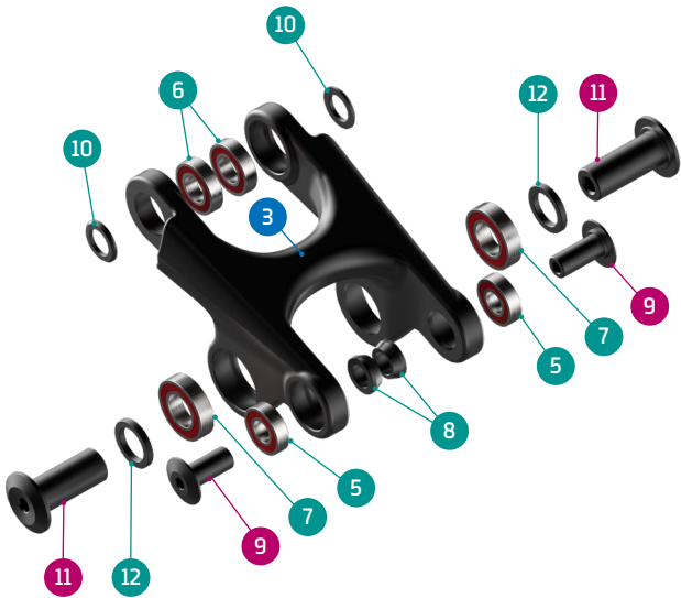
DETAIL 01
