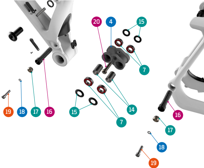
DETAIL 02
