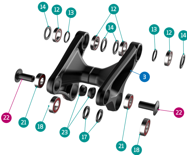
DETAIL 01
