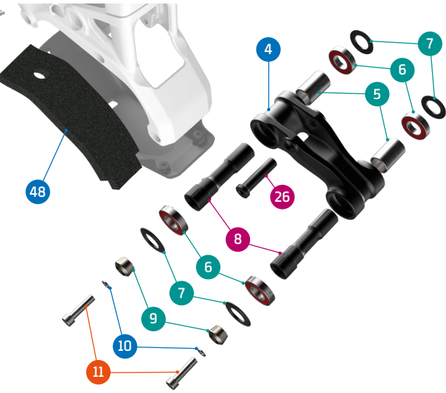
DETAIL 02
