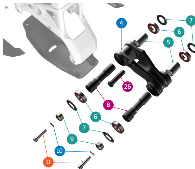
DETAIL 02
