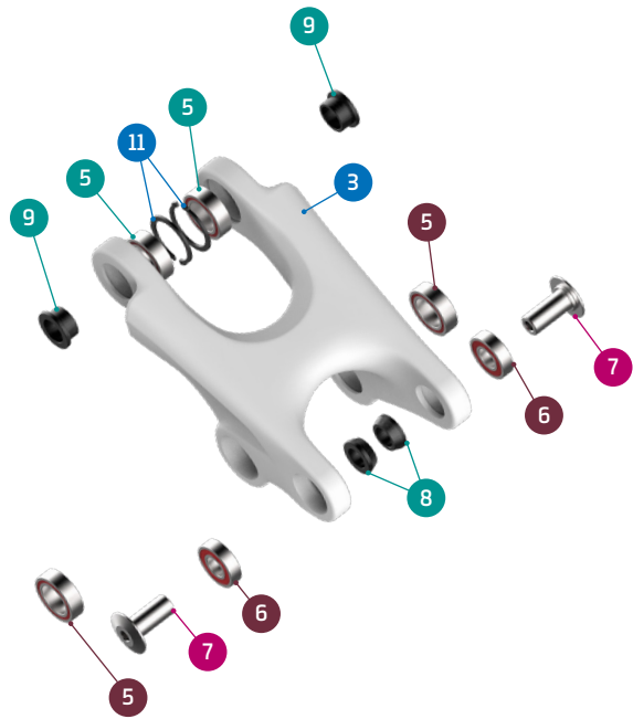
DETAIL 01
