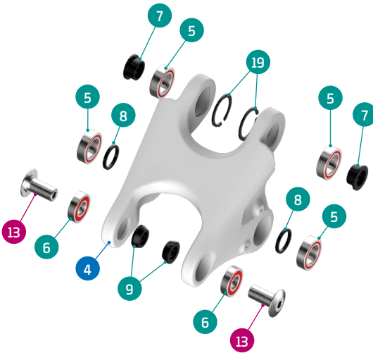
DETAIL 01
