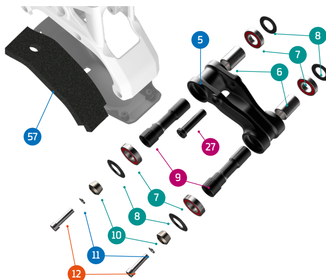
DETAIL 02
